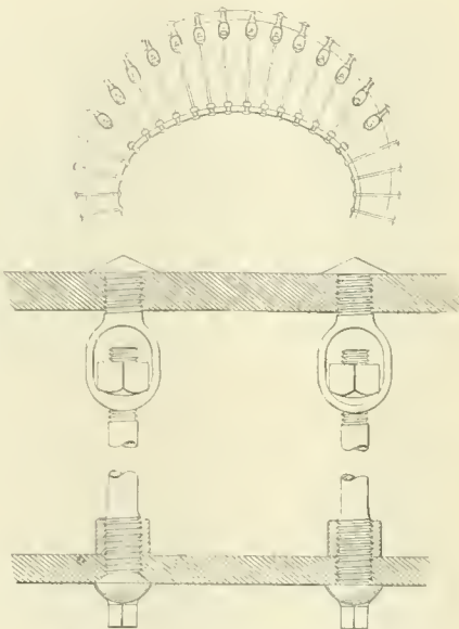
NEW RADIAL STAY FOR LOCOMOTIVE BOILERS.
